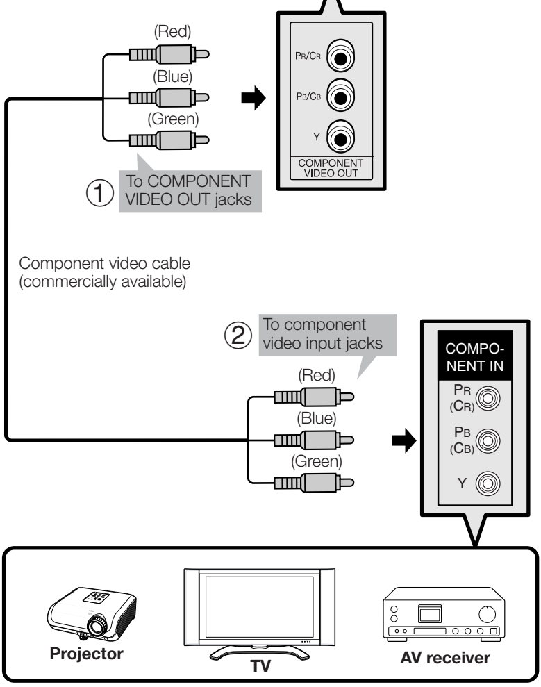
Video equipment with component jacks
